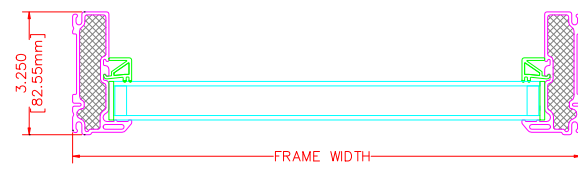
HORIZONTAL SECTION
