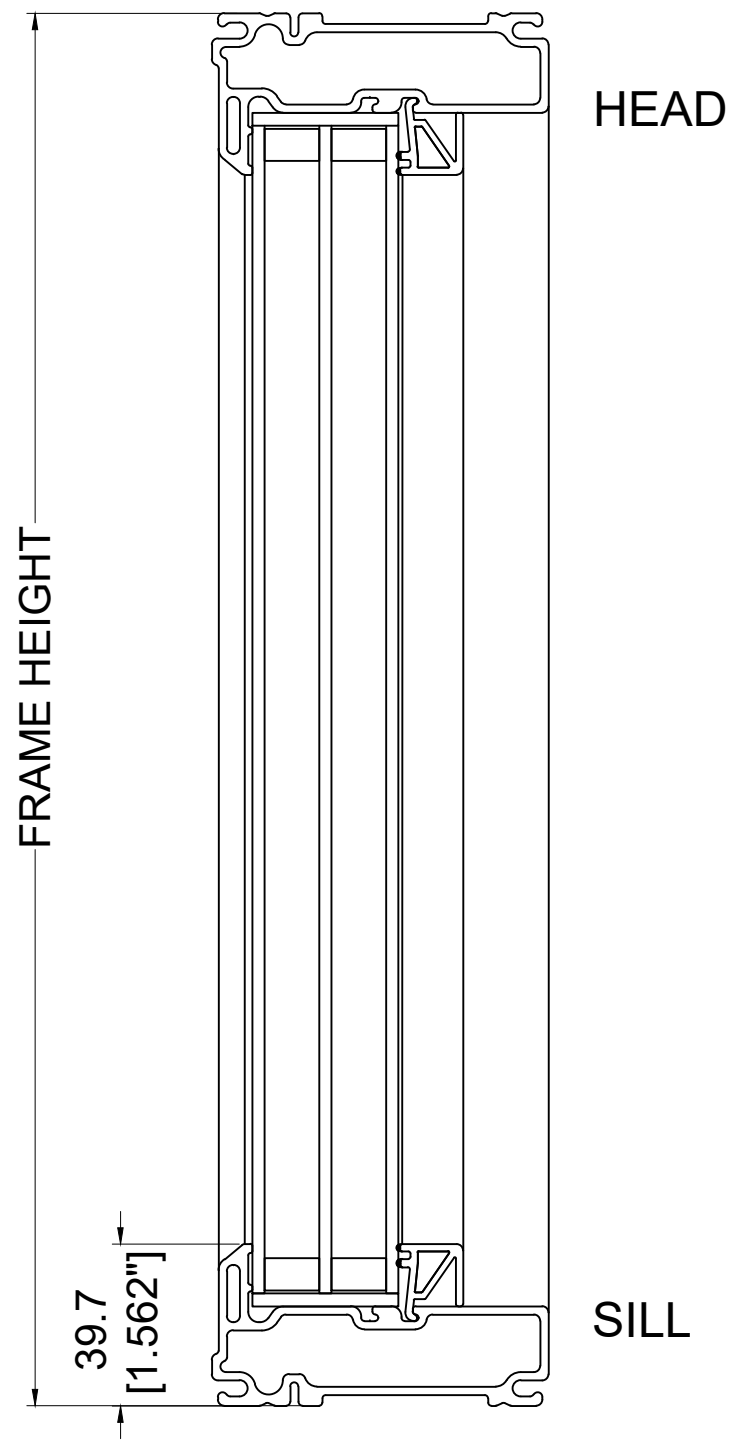
VERTICAL SECTION
