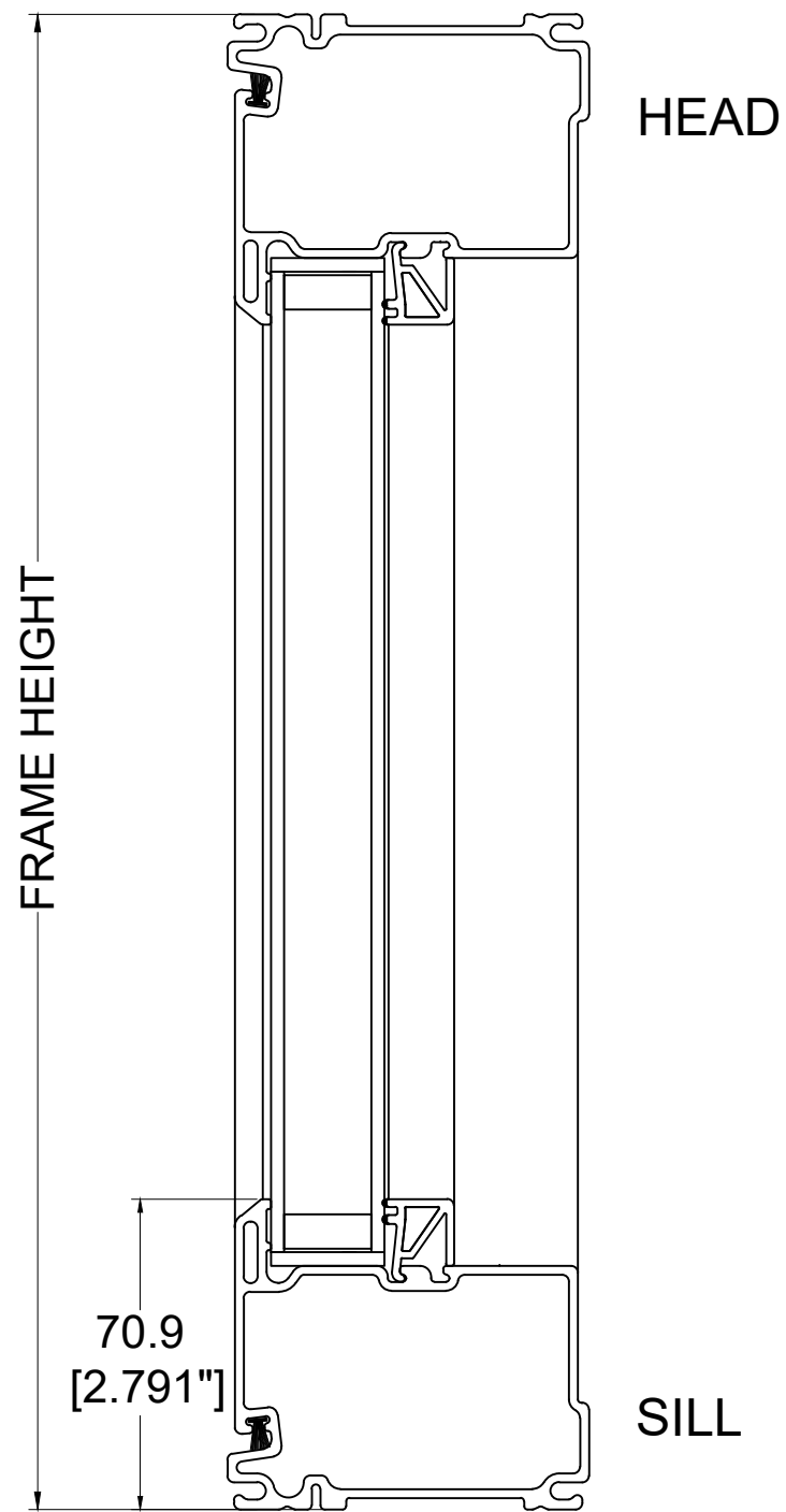
VERTICAL SECTION
