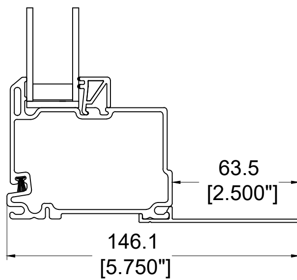
Anchor Bracket
